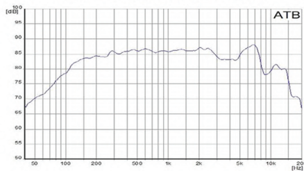
Frequenzgang / Frequency response [1W/1m]
