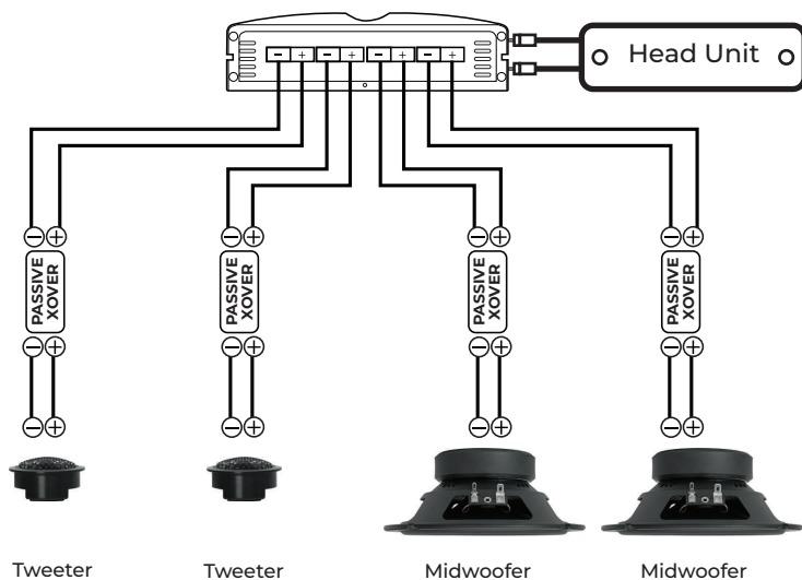
4 Channel Amplifier
