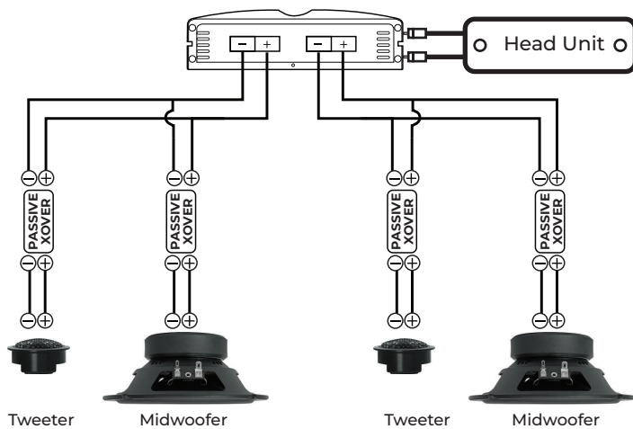
2 Channel Amplifier
