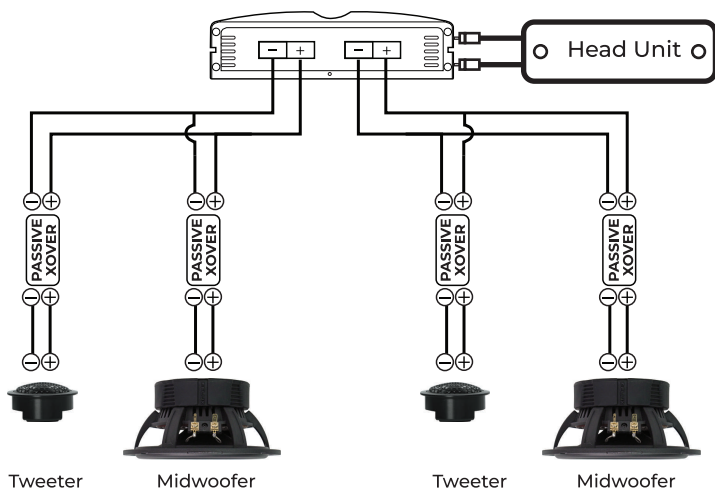
2 Channel Amplifier
