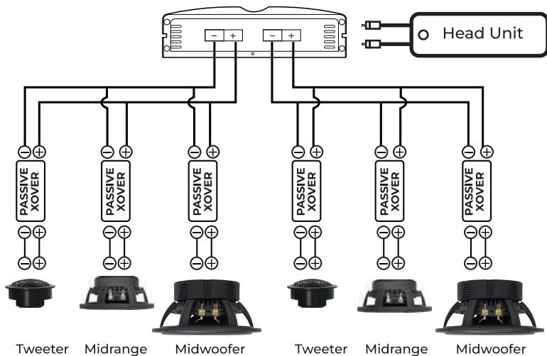
2 Channel Amplifier
