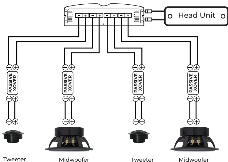
4 Channel Amplifier
